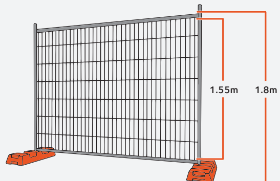
FIGURE 1 Standard Temporary Fence Measurements
